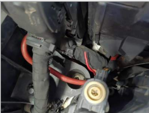
Engine Wiring
