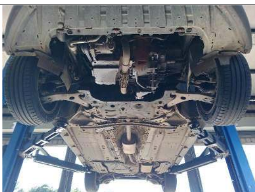
CHASSIS
